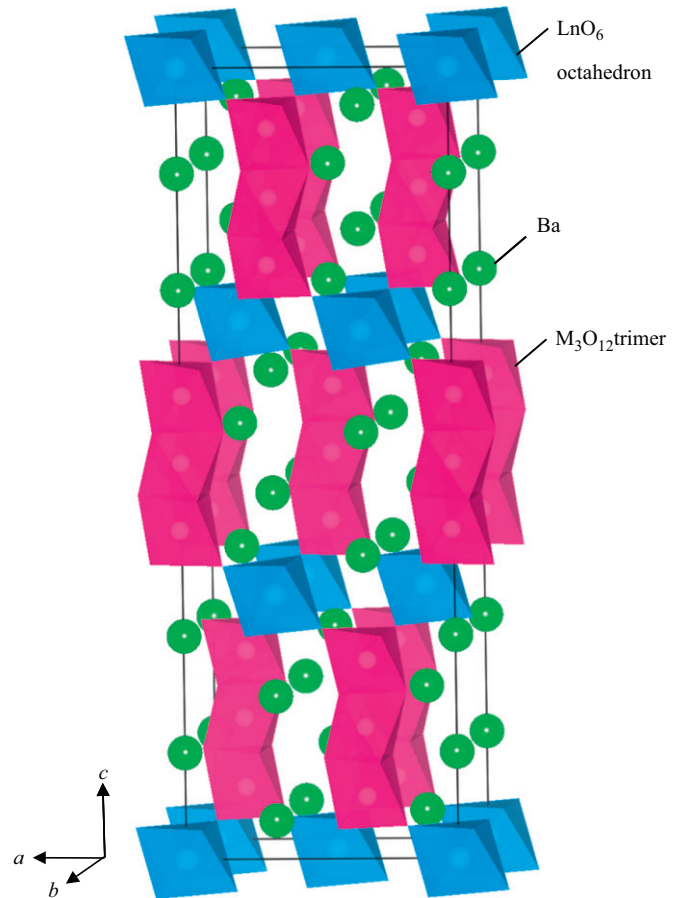
Fig. 2. The monoclinic perovskite structure with 12 layers for \text{Ba}_4\text{LnM}_3\text{O}_{12} ( \text{Ln}=\text{La}-\text{Gd} for M=\text{Ru} ; \text{Ln}=\text{La}-\text{Lu} for M=\text{Ir} ).
