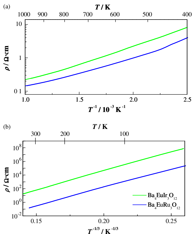
Fig.11. Temperature dependence of the resistivity for Ba_4EuM_3O_{12} ( M=Ru, Ir ). (a) \log \rho vs. T^{-1} plot and (b) \log \rho vs. T^{-1/3} plot.
