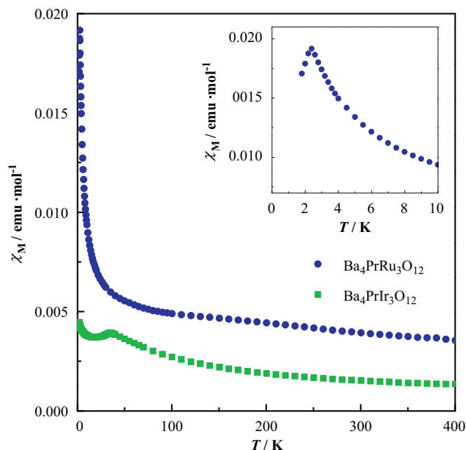
Fig. 7. Temperature dependence of the magnetic susceptibilities for \text{Ba}_4\text{PrM}_3\text{O}_{12} ( M=\text{Ru}, \text{Ir} ). The inset shows the magnetic susceptibilities of \text{Ba}_4\text{PrRu}_3\text{O}_{12} at low temperatures.
