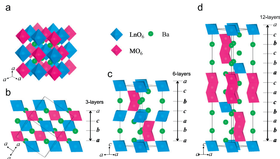
Fig. 1. Schematic crystal structures of (a) cubic double perovskite \text{Ba}_2\text{LnMO}_6 , (b) the stacking sequence of the double perovskite ( abc\dots ), (c) hexagonal triple perovskite \text{Ba}_3\text{LnM}_2\text{O}_9 (the stacking sequence: ababc\dots ), and (d) hexagonal quadruple perovskite \text{Ba}_4\text{LnM}_3\text{O}_{12} (the stacking sequence: ababcacabc\dots ).
