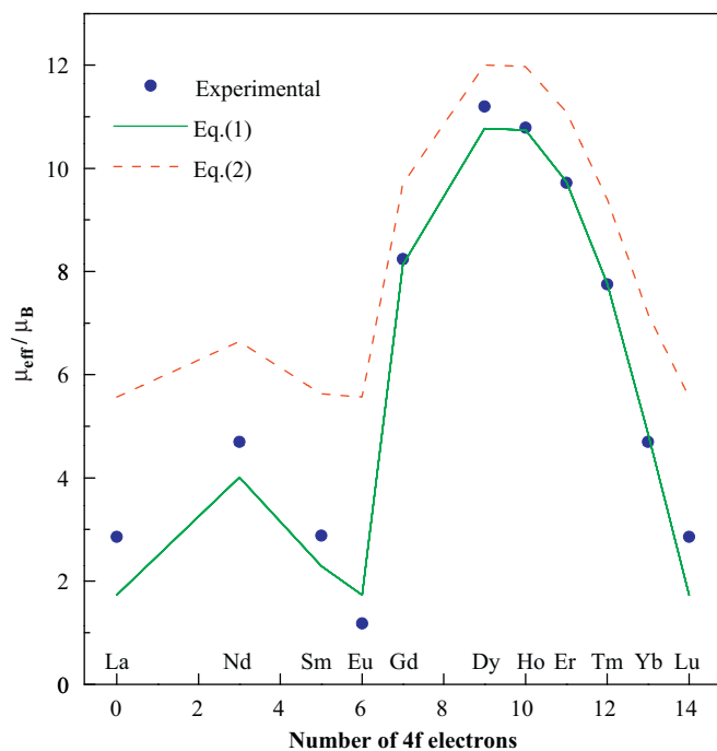
Fig. 9. Comparison of the effective magnetic moments of \text{Ba}_4\text{Ln}^{3+}\text{Ru}_3^{4.33+}\text{O}_{12} with the calculated values.
