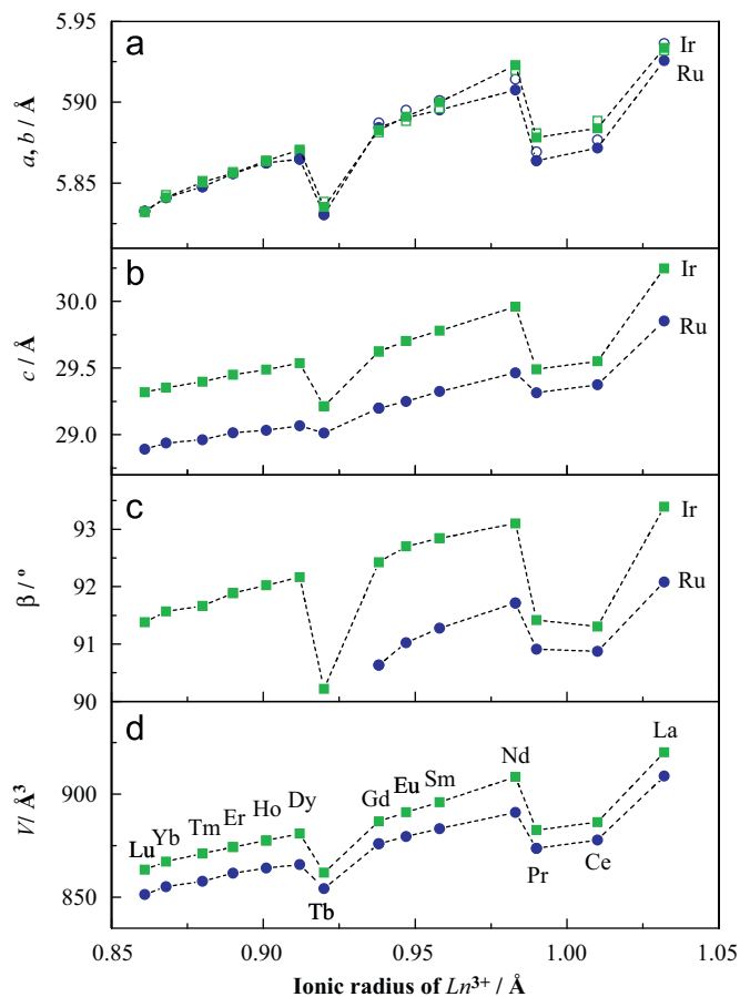
Fig. 3. Variation of lattice parameters and volumes for Ba_4LnM_3O_{12} against the ionic radius of Ln^{3+} ( M=Ru , circles; M=Ir , squares). (a) a (●, ■): for monoclinic structures, values of a/\sqrt{3} are plotted; b (○, □), (b) c , (c) \beta , and (d) volume V : for monoclinic structures, half of the volumes are plotted.
