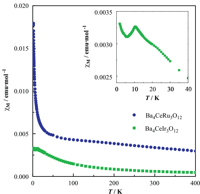
Fig. 6. Temperature dependence of the magnetic susceptibilities for \text{Ba}_4\text{CeM}_3\text{O}_{12} ( M=\text{Ru}, \text{Ir} ). The inset shows the magnetic susceptibilities of \text{Ba}_4\text{CeIr}_3\text{O}_{12} at low temperatures.
