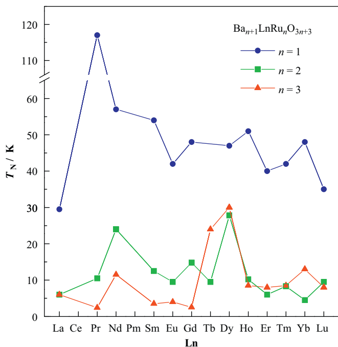
Fig.10. Magnetic transition temperatures of Ba_{n+1}LnRu_nO_{3n+3} .
