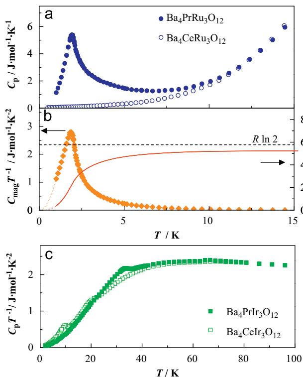
Fig. 8. (a) Temperature dependence of the specific heat ( C_p ) for \text{Ba}_4\text{LnRu}_3\text{O}_{12} ( \text{Ln}=\text{Ce}, \text{Pr} ). (b) The magnetic specific heat divided by temperature ( C_{\text{mag}}/T ) and the magnetic entropy ( S_m ) of \text{Ba}_4\text{PrRu}_3\text{O}_{12} . (c) Temperature dependence of the specific heat divided by temperature ( C_p/T ) for \text{Ba}_4\text{LnIr}_3\text{O}_{12} ( \text{Ln}=\text{Ce}, \text{Pr} ).
