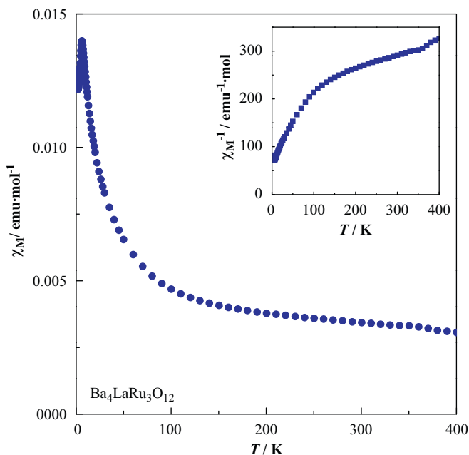
Fig. 5. Temperature dependence of the magnetic susceptibility for \text{Ba}_4\text{LaRu}_3\text{O}_{12} . The inset shows the reciprocal susceptibility against temperature.
